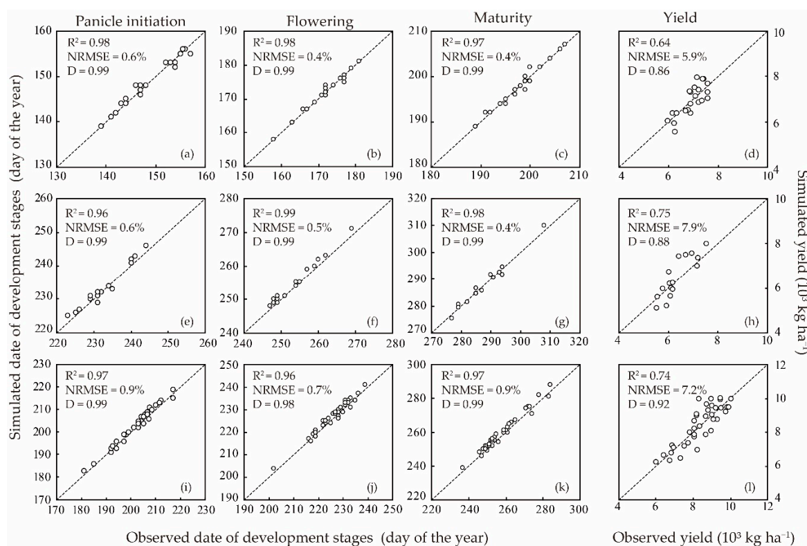
Figure 2. Comparison of the simulated and observed date of panicle initiation (a,e,i), flowering (b,f,j), physiological maturity (c,g,k), and grain yield (d,h,l) for early rice (a–d), late rice (e–h) and middle rice (i–l). The dashed line represents the 1:1 line.
