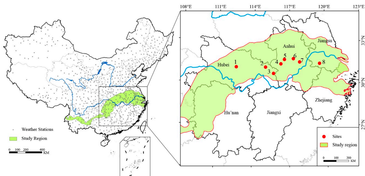
Figure 1. The study region, the selected 8 rice experimental sites (Red dots), and the locations of meteorological stations (black points) in the middle and lower reaches of the Yangtze River in China.
