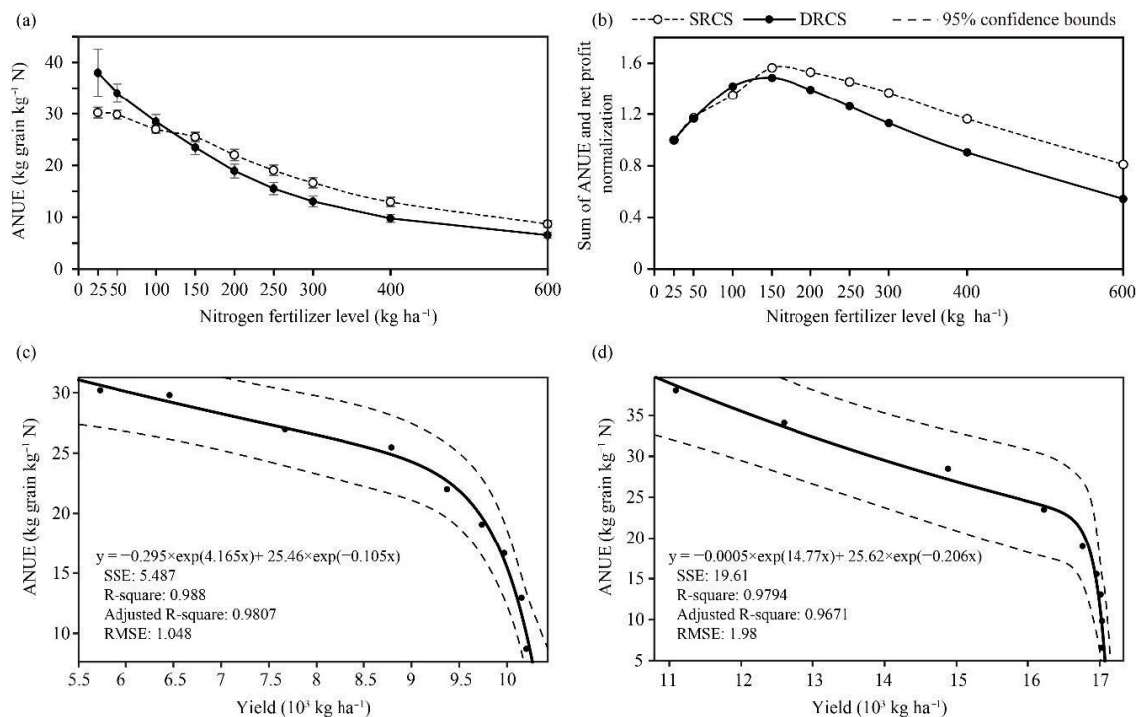
Figure 6. Relationships between agronomic nitrogen use efficiency (ANUE) and nitrogen fertilizer levels, rice grain yield, and net profit for SRCS and DRCS in the study region. Note: Dotted lines are the 95% confidence bounds. (a) ANUE vs. nitrogen fertilizer level for SRCS and DRCS. (b) Sum of ANUE and net profit normalization vs. nitrogen fertilizer level for SRCS and DRCS. (c) ANUE vs. rice grain yield for SRCS. (d) ANUE vs. rice grain yield for DRCS.
