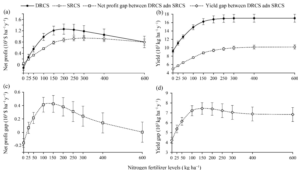
Figure 4. Net profit ( \$ \text{ha}^{-1} \text{y}^{-1} ) (a) and rice grain yield ( \text{kg ha}^{-1} \text{y}^{-1} ) (b) for DRCS and SRCS at different nitrogen fertilizer levels during the growing season ( \text{kg ha}^{-1} ) from 1981 to 2015. Note: Error bars indicate the standard deviations. (c) Net profit gap between DRCS and SRCS. (d) Rice grain yield gap between DRCS and SRCS.
