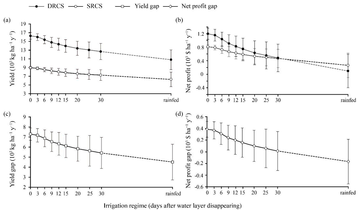
Figure 5. Rice grain yield ( 10^3 \text{ kg ha}^{-1} \text{ y}^{-1} ) (a) and net profit ( 10^3 \text{ \$ ha}^{-1} \text{ y}^{-1} ) (b) for DRCS and SRCS at different irrigation regimes, including rainfed condition (i.e., no irrigation), during the growing season from 1981 to 2015. Note: Error bars indicate the standard deviations. (c) Rice grain yield gap between DRCS and SRCS. (d) Net profit gap between DRCS and SRCS.
